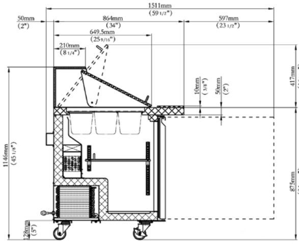
SECTION VIEW
